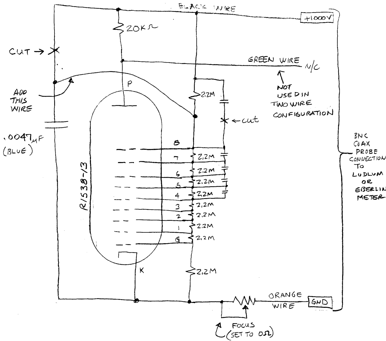
R1538-13 CONNECTION FOR SCINTILLATION PROBE 2-WIRE
